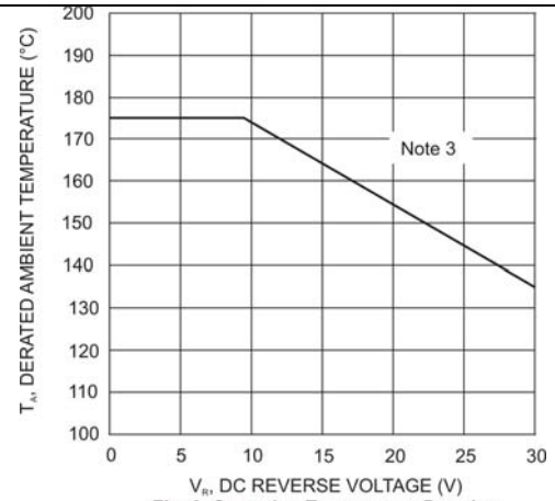
Fig. 6 Operating Temperature Derating
