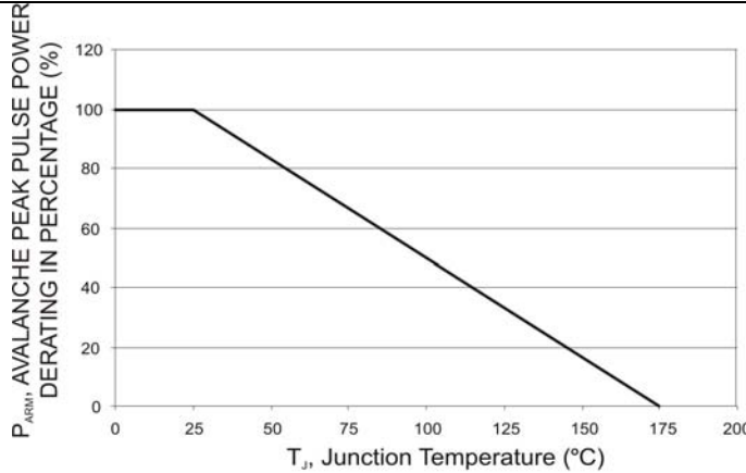
Fig. 7: Pulse Derating Curve, Per Element
