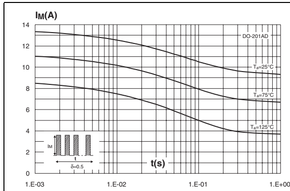
Figure 5. Non repetitive surge peak forward current versus overload duration (maximum values) (DO-201AD)
