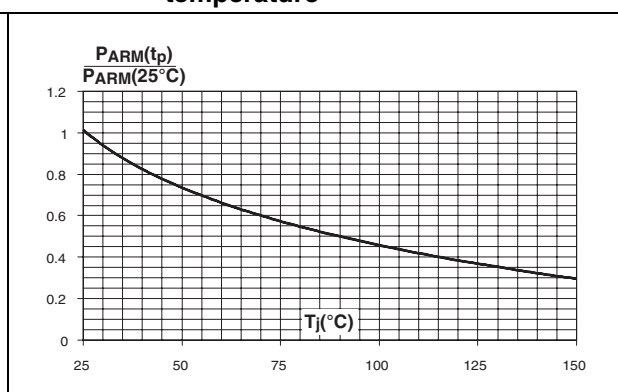
Figure 8. Normalized avalanche power derating versus junction temperature
