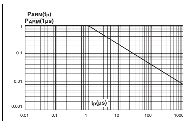
Figure 7. Normalized avalanche power derating versus pulse duration
