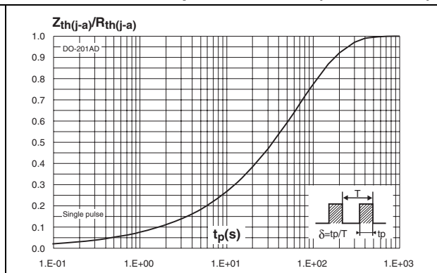
Figure 10. Relative variation of thermal impedance junction to ambient versus pulse duration (DO-201AD)
