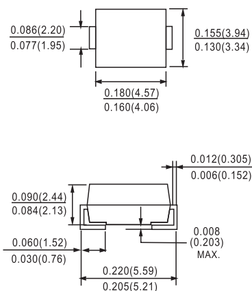
DO-214AA(SMB)
