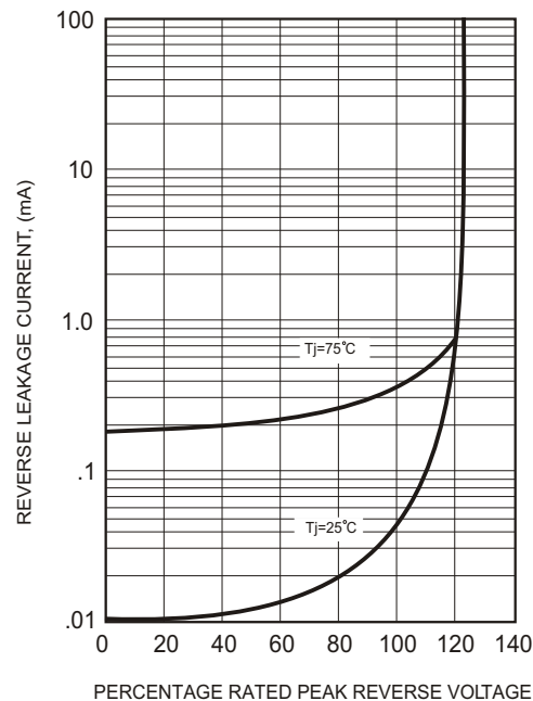
FIG.5 - TYPICAL REVERSE
