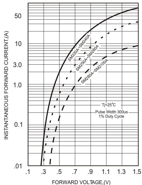
FIG.2-TYPICAL FORWARD
