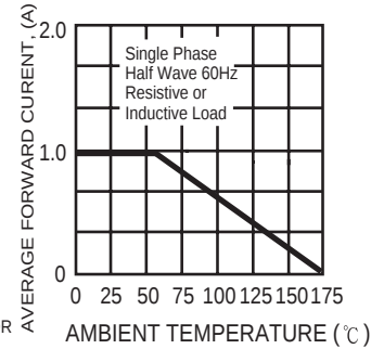
FIG. 2 - TYPICAL FORWARD CURRENT DERATING CURVE
