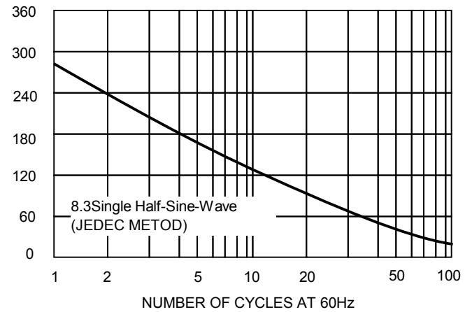
FIG.2-MAXIMUM NON-REPETITIVE SURGE
