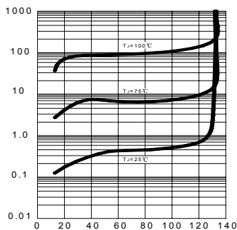
FIG.6 -- TYPICAL REVERSE CHARACTERISTICS
